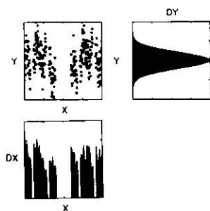
Figure 7. From a Cantorian multifractal measure to the Gaussian via a fractal interpolator. Data points \{(0,0), (0.2, 1), (0.4, -1), (0.6, -1), (0.8, 1), (1, 0)\} ; p_1 = 0.3, p_2 = 0.2, p_3 = 0, p_4 = 0.25, p_5 = 0.25 ; d_1 = -d_2 = d_3 = d_4 = -d_5 = 0.995 .
