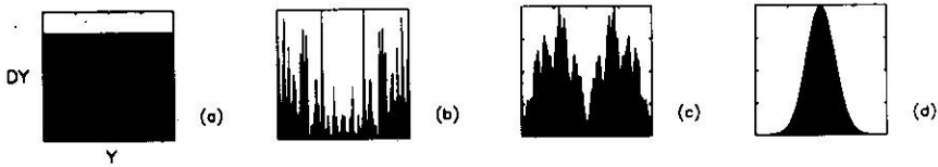
Figure 3. Derived measures Y = f_z(U) for the fractal interpolators in Figure 2.
