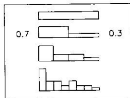
Figure 4. Geometric construction of binomial multifractal measure.
